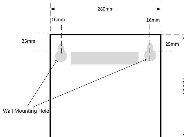
Figure 2. Product Mounting
