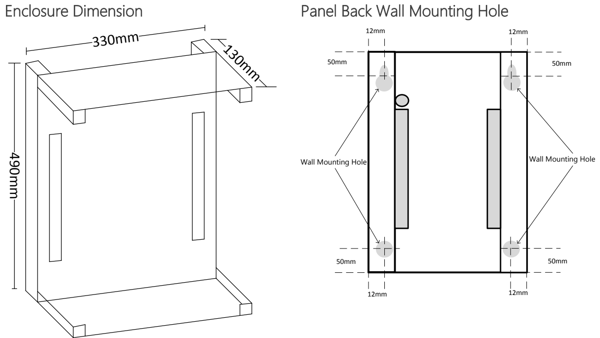
Figure 1. Product Mounting
